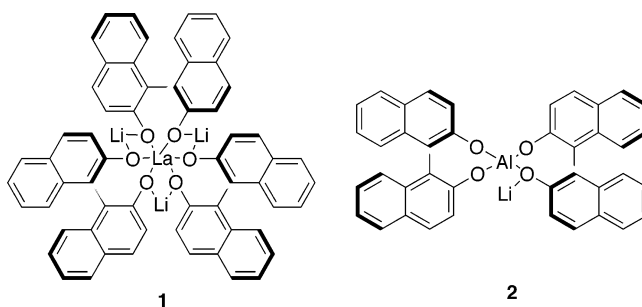
FIGURE 1. LaLi 3 tris(binaphthoxide) catalyst 1 and AlLi 3 bis(binaphthoxide) (ALB) 2 .
